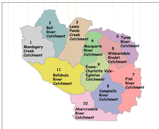
CTLD Sub-Catchments
